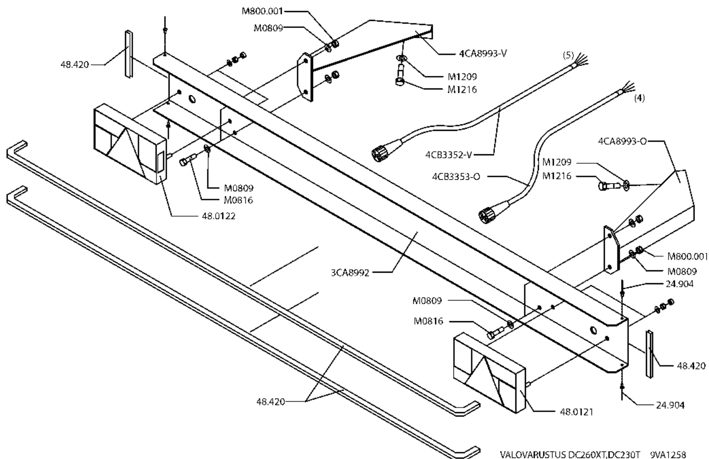
VALOVARUSTUS DC260XT,DC230T 9VA1258
