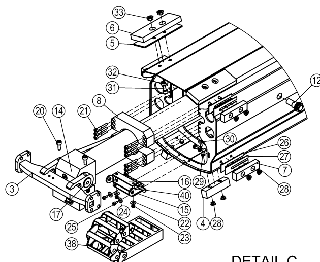
DETAIL C
